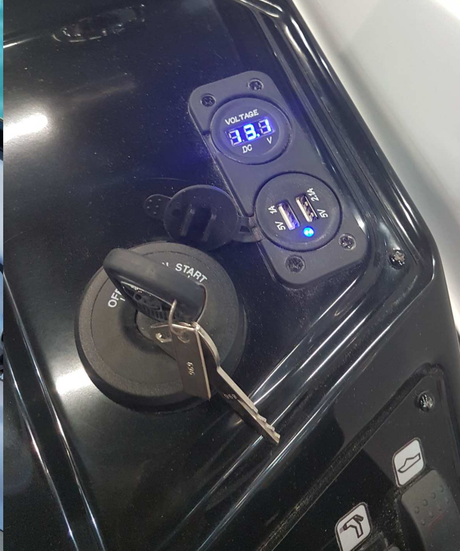
Sport helm station with two USB inputs and digital voltmeter
